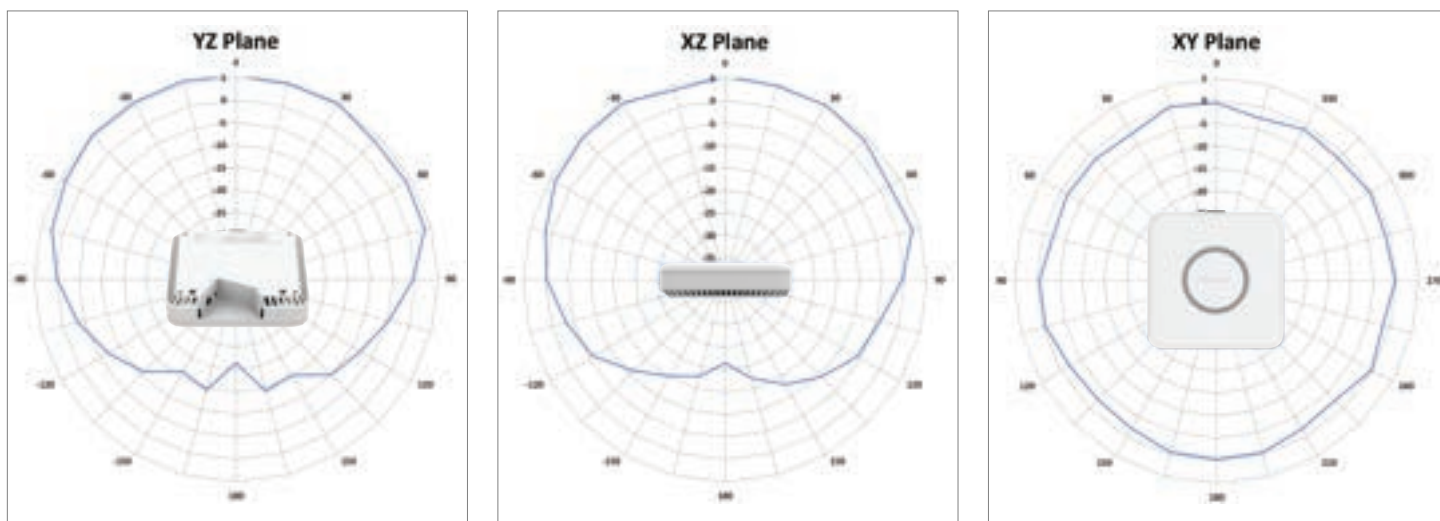
Radio Pattern for 6GHz
