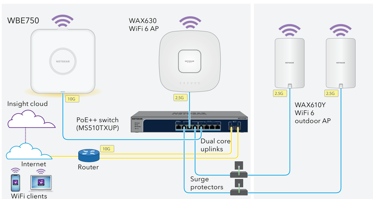
WBE750 Deployment Scenario
