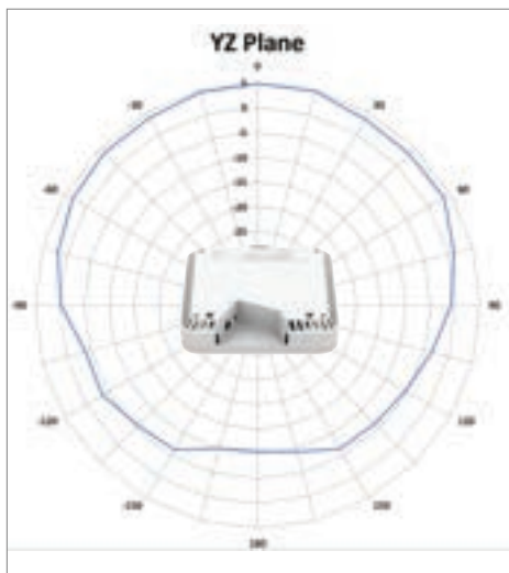
Radio Pattern for 5GHz
