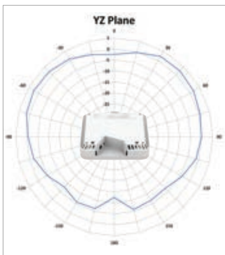
Radio Pattern for 2.4GHz
